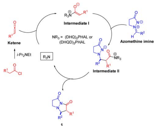
Scheme 2. Proposed Mechanism for Catalytic Asymmetric Synthesis of Bicyclic Pyrazolidinones
