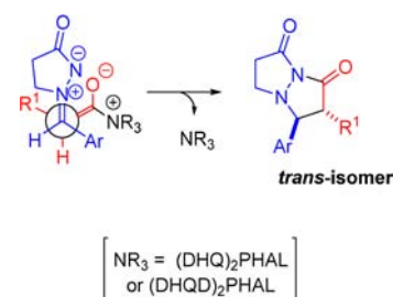
Scheme 3. Model for Diastereoselection
