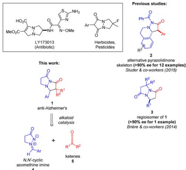
Scheme 1. Plan for Synthesis of Bicyclic Pyrazolidinones
